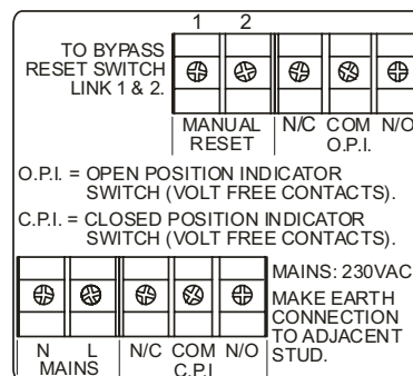
TERMINAL BLOCK WIRING
